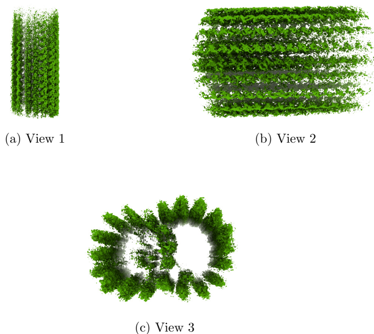
Figure 4: Isosurface at threshold=0.353000. Views generated by ChimeraX at a the following X, Y, Z angles: View 1 (0, -90, -90), View 2 (-90, 0, -90), View 3 (0, 0, 0).
