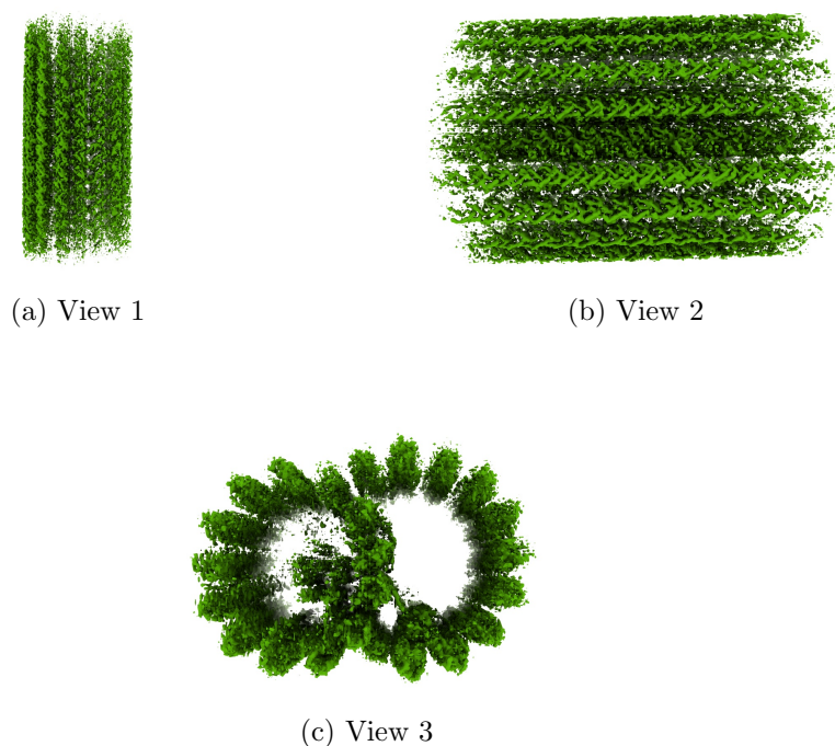
Figure 4: Isosurface at threshold=0.439000. Views generated by ChimeraX at a the following X, Y, Z angles: View 1 (0, -90, -90), View 2 (-90, 0, -90), View 3 (0, 0, 0).
