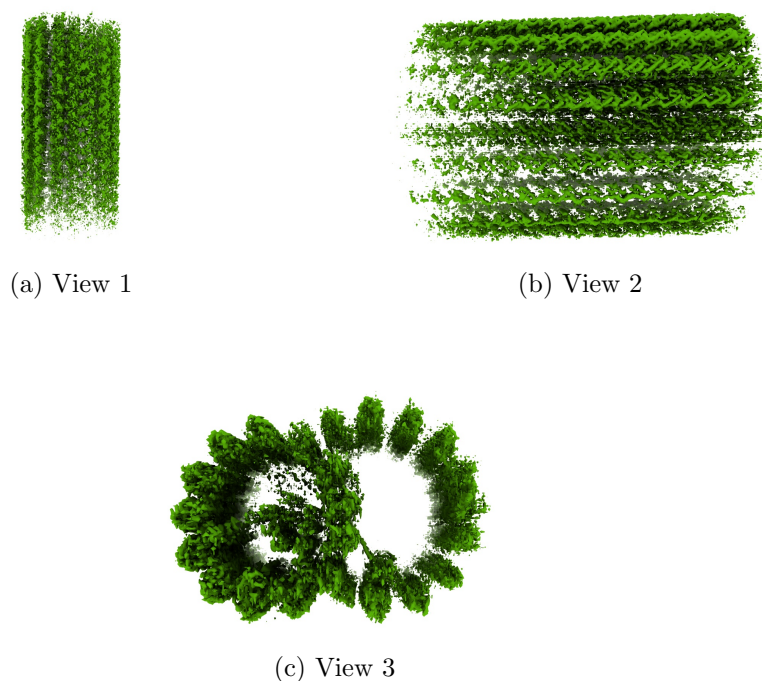
Figure 4: Isosurface at threshold=0.390000. Views generated by ChimeraX at a the following X, Y, Z angles: View 1 (0, -90, -90), View 2 (-90, 0, -90), View 3 (0, 0, 0).
