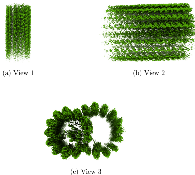
Figure 4: Isosurface at threshold=0.386000. Views generated by ChimeraX at a the following X, Y, Z angles: View 1 (0, -90, -90), View 2 (-90, 0, -90), View 3 (0, 0, 0).
