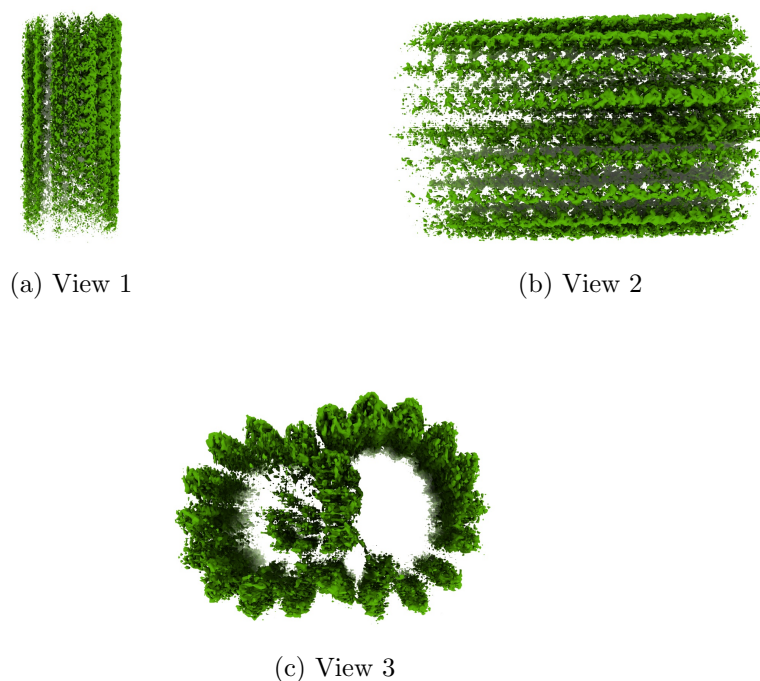
Figure 4: Isosurface at threshold=0.349000. Views generated by ChimeraX at a the following X, Y, Z angles: View 1 (0, -90, -90), View 2 (-90, 0, -90), View 3 (0, 0, 0).
