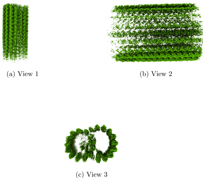
Figure 4: Isosurface at threshold=0.325000. Views generated by ChimeraX at a the following X, Y, Z angles: View 1 (0, -90, -90), View 2 (-90, 0, -90), View 3 (0, 0, 0).
