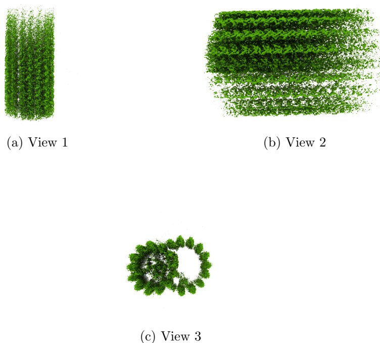
Figure 4: Isosurface at threshold=0.468000. Views generated by ChimeraX at a the following X, Y, Z angles: View 1 (0, -90, -90), View 2 (-90, 0, -90), View 3 (0, 0, 0).
