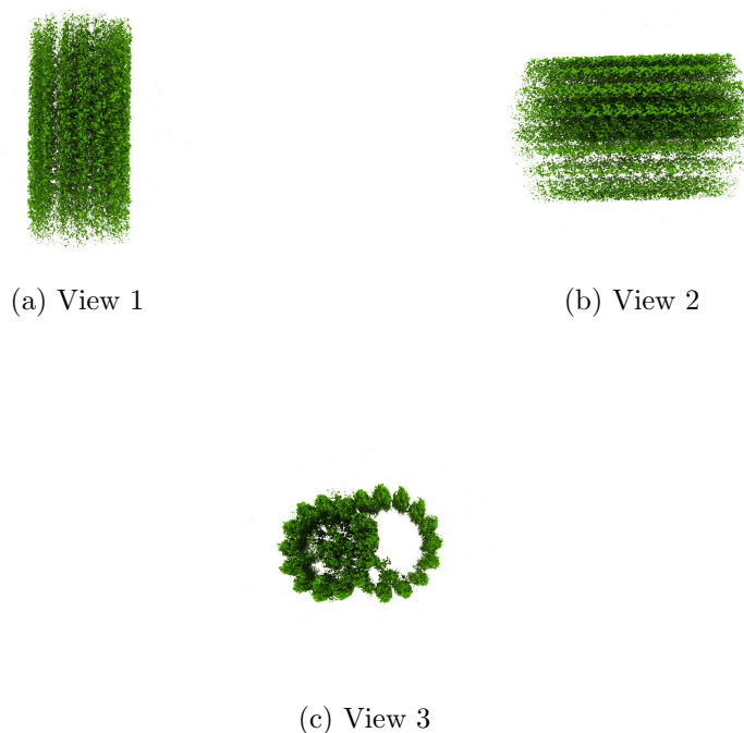
Figure 4: Isosurface at threshold=0.545000. Views generated by ChimeraX at a the following X, Y, Z angles: View 1 (0, -90, -90), View 2 (-90, 0, -90), View 3 (0, 0, 0).
