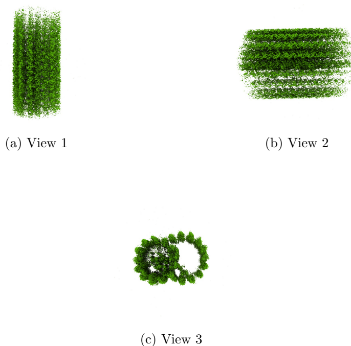
Figure 4: Isosurface at threshold=0.452000. Views generated by ChimeraX at a the following X, Y, Z angles: View 1 (0, -90, -90), View 2 (-90, 0, -90), View 3 (0, 0, 0).
