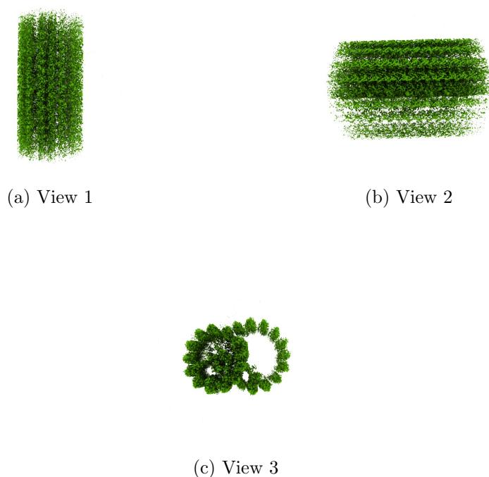
Figure 4: Isosurface at threshold=0.562000. Views generated by ChimeraX at a the following X, Y, Z angles: View 1 (0, -90, -90), View 2 (-90, 0, -90), View 3 (0, 0, 0).
