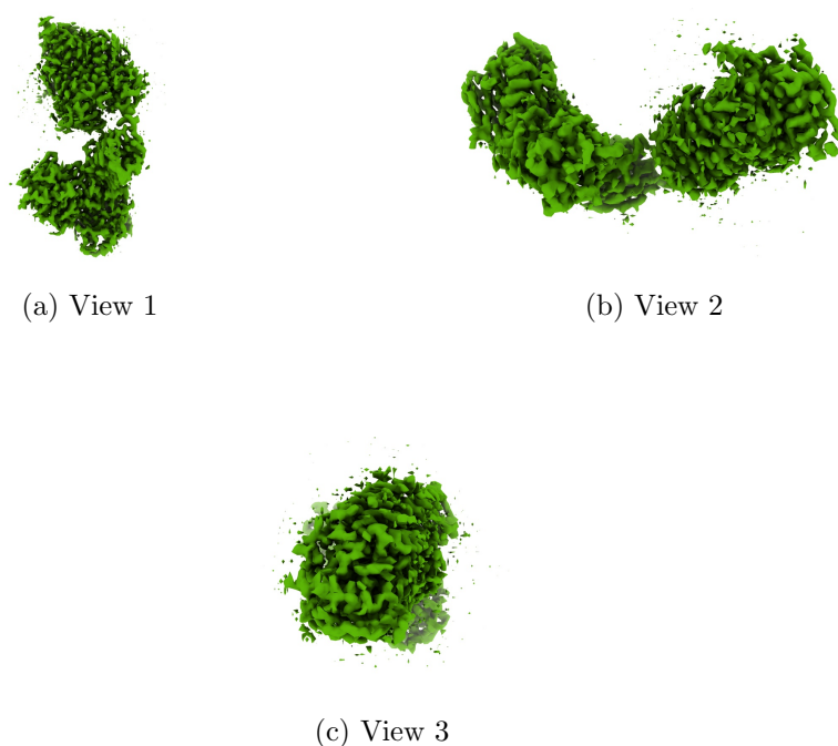
Figure 4: Isosurface at threshold=4.410000. Views generated by ChimeraX at a the following X, Y, Z angles: View 1 (0, -90, -90), View 2 (-90, 0, -90), View 3 (0, 0, 0).
