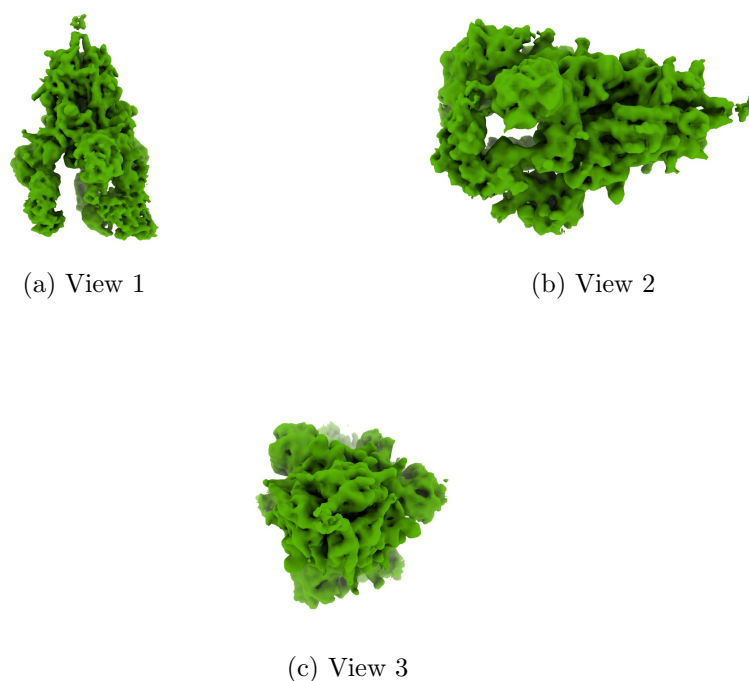
Figure 4: Isosurface at threshold=0.175000. Views generated by ChimeraX at a the following X, Y, Z angles: View 1 (0, -90, -90), View 2 (-90, 0, -90), View 3 (0, 0, 0).
