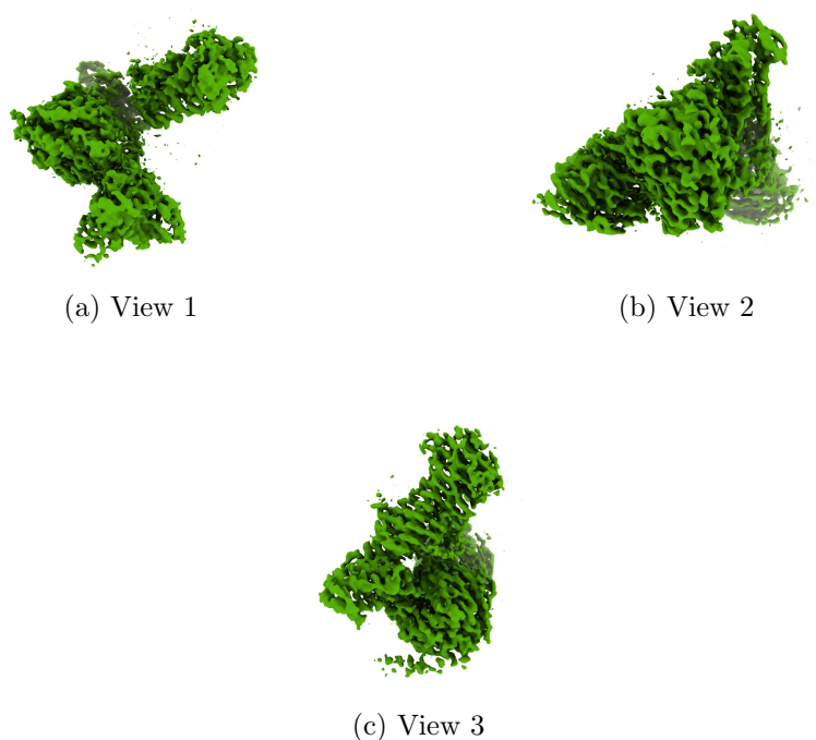
Figure 4: Isosurface at threshold=0.626000. Views generated by ChimeraX at a the following X, Y, Z angles: View 1 (0, -90, -90), View 2 (-90, 0, -90), View 3 (0, 0, 0).
