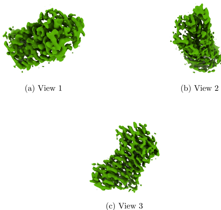
Figure 4: Isosurface at threshold=0.904000. Views generated by ChimeraX at a the following X, Y, Z angles: View 1 (0, -90, -90), View 2 (-90, 0, -90), View 3 (0, 0, 0).
