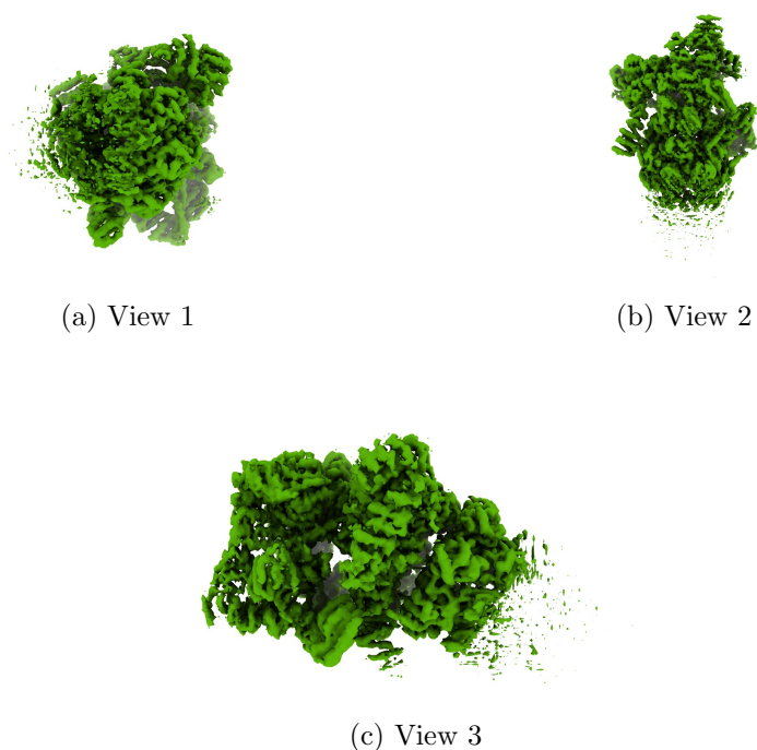
Figure 4: Isosurface at threshold=5.500000. Views generated by ChimeraX at a the following X, Y, Z angles: View 1 (0, -90, -90), View 2 (-90, 0, -90), View 3 (0, 0, 0).
