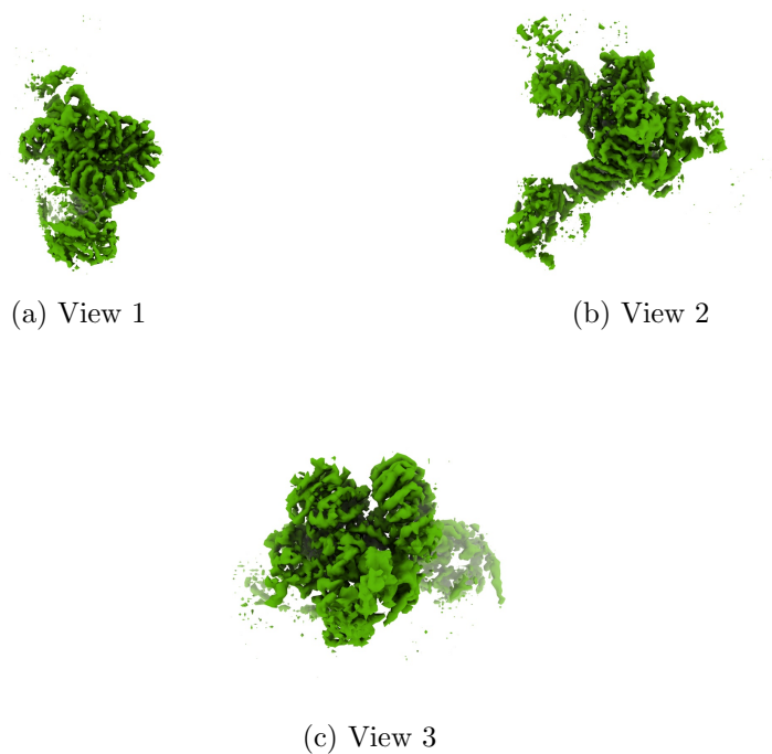
Figure 4: Isosurface at threshold=0.038000. Views generated by ChimeraX at a the following X, Y, Z angles: View 1 (0, -90, -90), View 2 (-90, 0, -90), View 3 (0, 0, 0).
