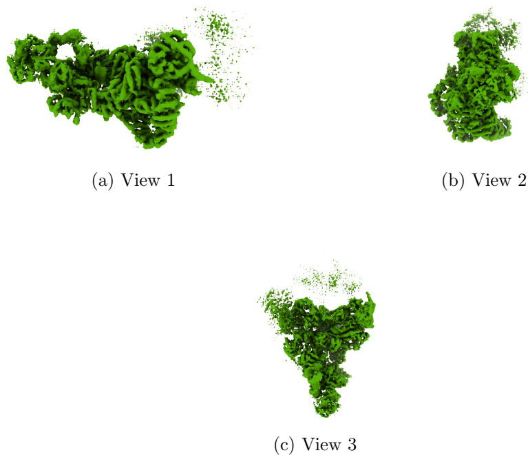
Figure 4: Isosurface at threshold=0.034800. Views generated by ChimeraX at a the following X, Y, Z angles: View 1 (0, -90, -90), View 2 (-90, 0, -90), View 3 (0, 0, 0).
