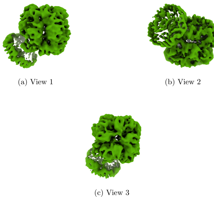
Figure 4: Isosurface at threshold=0.052400. Views generated by ChimeraX at a the following X, Y, Z angles: View 1 (0, -90, -90), View 2 (-90, 0, -90), View 3 (0, 0, 0).
