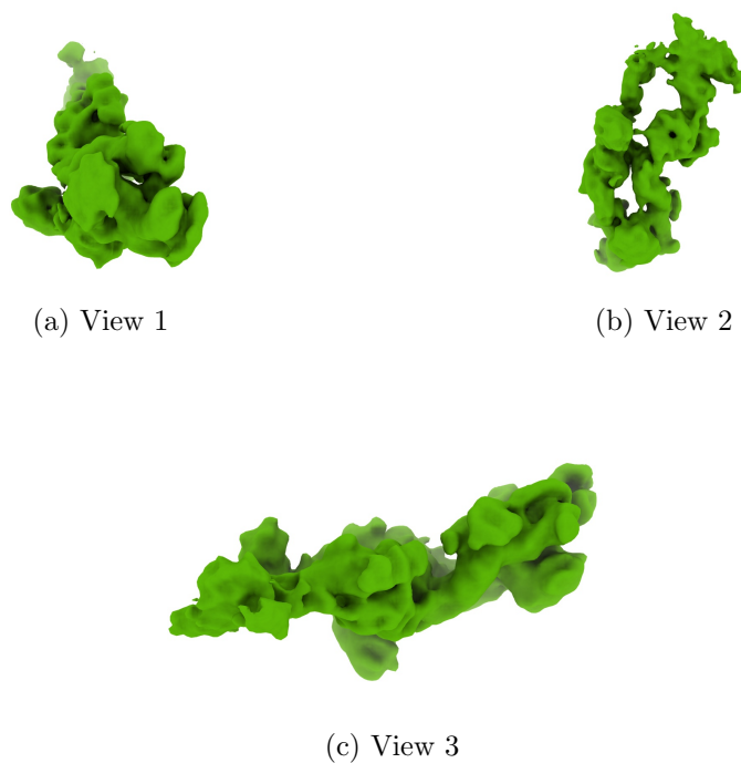
Figure 4: Isosurface at threshold=0.060000. Views generated by ChimeraX at a the following X, Y, Z angles: View 1 (0, -90, -90), View 2 (-90, 0, -90), View 3 (0, 0, 0).
