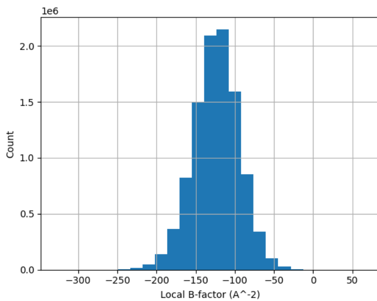
Figure 12: Histogram of the local B-factor according to LocBfactor.
