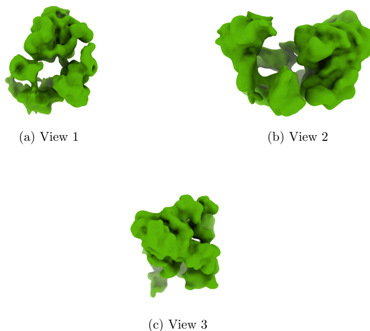
Figure 4: Isosurface at threshold=0.633000. Views generated by ChimeraX at a the following X, Y, Z angles: View 1 (0, -90, -90), View 2 (-90, 0, -90), View 3 (0, 0, 0).
