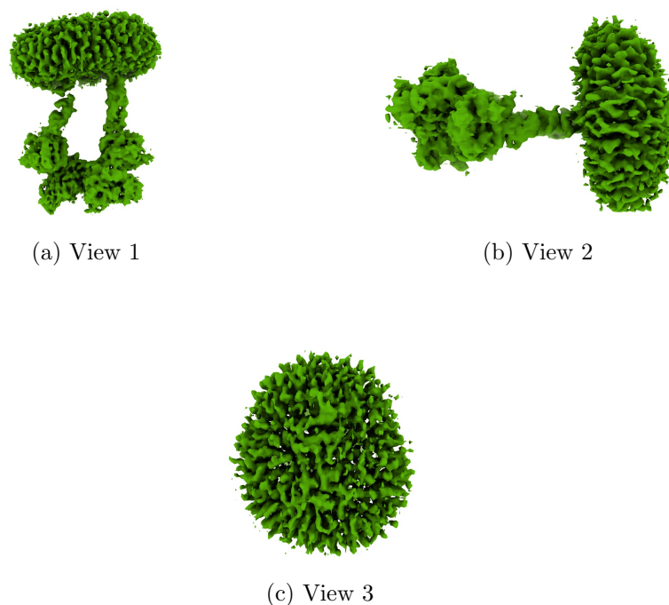
Figure 4: Isosurface at threshold=0.209000. Views generated by ChimeraX at a the following X, Y, Z angles: View 1 (0, -90, -90), View 2 (-90, 0, -90), View 3 (0, 0, 0).
