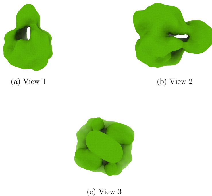
Figure 4: Isosurface at threshold=0.104700. Views generated by ChimeraX at a the following X, Y, Z angles: View 1 (0, -90, -90), View 2 (-90, 0, -90), View 3 (0, 0, 0).
