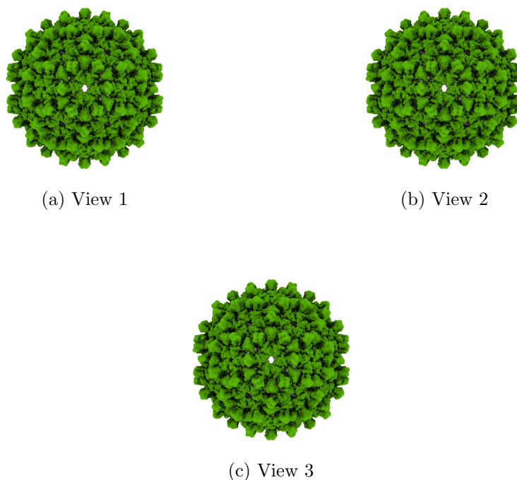
Figure 4: Isosurface at threshold=0.023200. Views generated by ChimeraX at a the following X, Y, Z angles: View 1 (0, -90, -90), View 2 (-90, 0, -90), View 3 (0, 0, 0).
