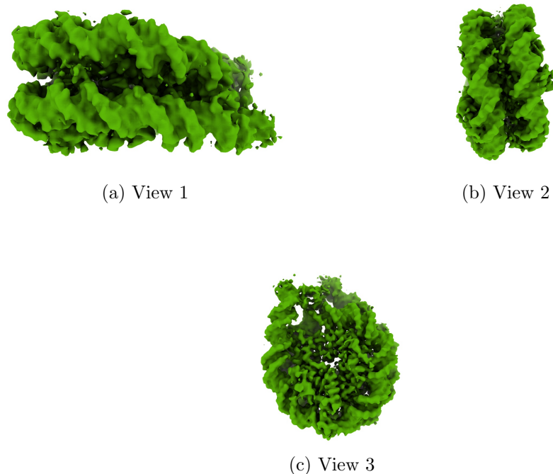
Figure 4: Isosurface at threshold=0.268000. Views generated by ChimeraX at a the following X, Y, Z angles: View 1 (0, -90, -90), View 2 (-90, 0, -90), View 3 (0, 0, 0).
