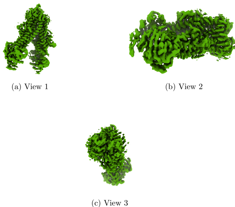
Figure 4: Isosurface at threshold=0.068000. Views generated by ChimeraX at a the following X, Y, Z angles: View 1 (0, -90, -90), View 2 (-90, 0, -90), View 3 (0, 0, 0).
