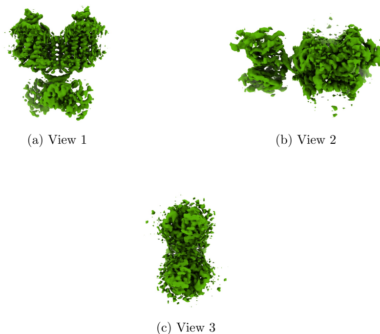
Figure 4: Isosurface at threshold=0.088100. Views generated by ChimeraX at a the following X, Y, Z angles: View 1 (0, -90, -90), View 2 (-90, 0, -90), View 3 (0, 0, 0).
