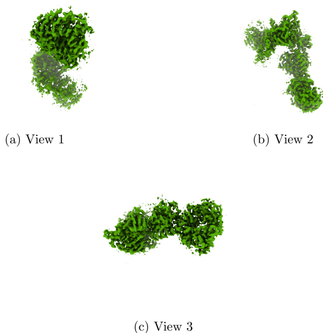
Figure 4: Isosurface at threshold=0.160000. Views generated by ChimeraX at a the following X, Y, Z angles: View 1 (0, -90, -90), View 2 (-90, 0, -90), View 3 (0, 0, 0).
