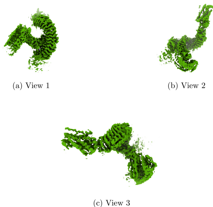
Figure 4: Isosurface at threshold=0.163000. Views generated by ChimeraX at a the following X, Y, Z angles: View 1 (0, -90, -90), View 2 (-90, 0, -90), View 3 (0, 0, 0).
