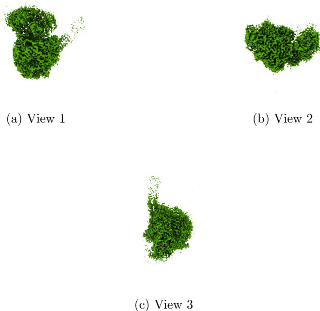
Figure 4: Isosurface at threshold=0.097700. Views generated by ChimeraX at a the following X, Y, Z angles: View 1 (0, -90, -90), View 2 (-90, 0, -90), View 3 (0, 0, 0).
