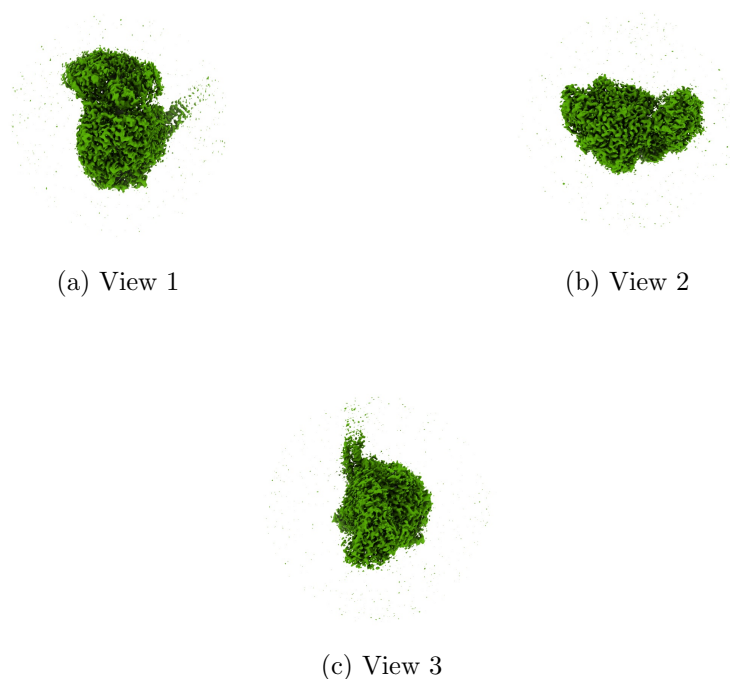
Figure 4: Isosurface at threshold=0.078000. Views generated by ChimeraX at a the following X, Y, Z angles: View 1 (0, -90, -90), View 2 (-90, 0, -90), View 3 (0, 0, 0).
