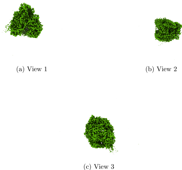
Figure 4: Isosurface at threshold=0.109000. Views generated by ChimeraX at a the following X, Y, Z angles: View 1 (0, -90, -90), View 2 (-90, 0, -90), View 3 (0, 0, 0).
