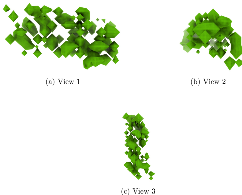
Figure 4: Isosurface at threshold=0.140000. Views generated by ChimeraX at a the following X, Y, Z angles: View 1 (0, -90, -90), View 2 (-90, 0, -90), View 3 (0, 0, 0).
