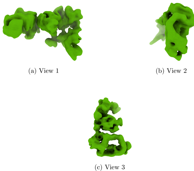
Figure 4: Isosurface at threshold=0.002890. Views generated by ChimeraX at a the following X, Y, Z angles: View 1 (0, -90, -90), View 2 (-90, 0, -90), View 3 (0, 0, 0).
