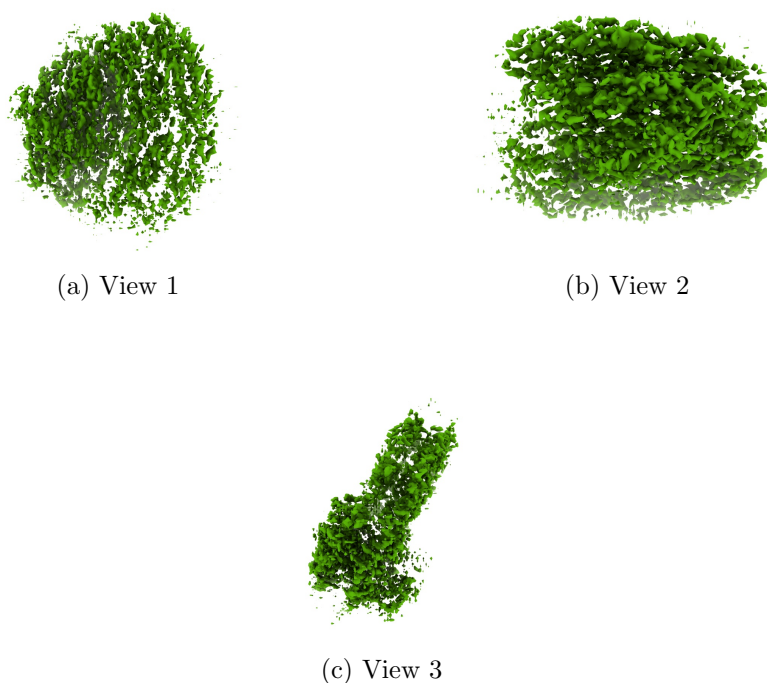
Figure 4: Isosurface at threshold=0.809000. Views generated by ChimeraX at a the following X, Y, Z angles: View 1 (0, -90, -90), View 2 (-90, 0, -90), View 3 (0, 0, 0).
