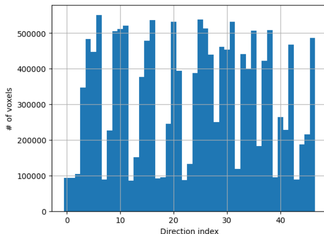
Figure 29: Histogram 1D of the best direction at each voxel.
