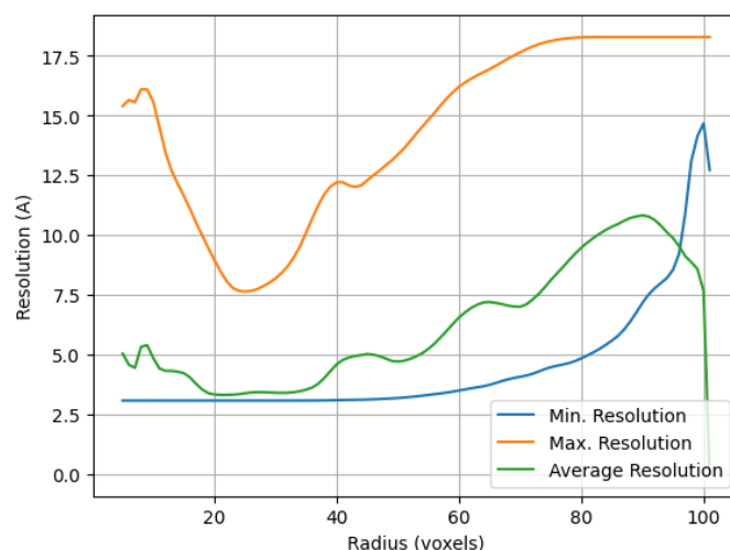
Figure 30: Radial averages (in space) of the minimum, maximum and average resolution at each voxel.
