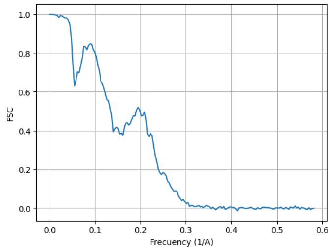
Figure 21: FSC and resolution estimated by a permutation test.
