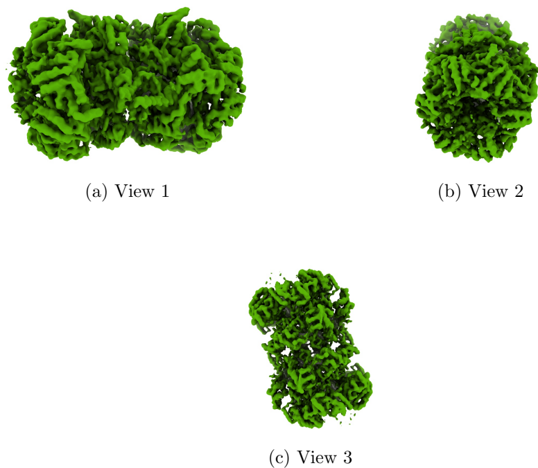
Figure 4: Isosurface at threshold=0.878000. Views generated by ChimeraX at a the following X, Y, Z angles: View 1 (0, -90, -90), View 2 (-90, 0, -90), View 3 (0, 0, 0).
