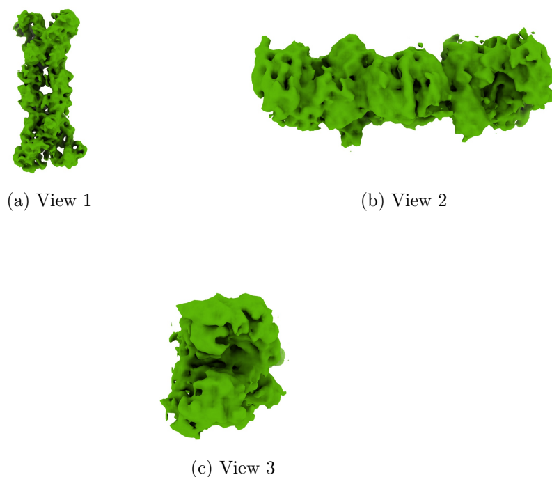
Figure 4: Isosurface at threshold=0.700000. Views generated by ChimeraX at the following X, Y, Z angles: View 1 (0, -90, -90), View 2 (-90, 0, -90), View 3 (0, 0, 0).
