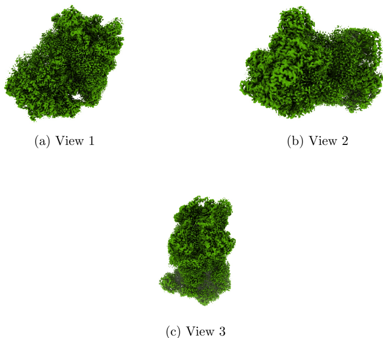
Figure 4: Isosurface at threshold=0.009430. Views generated by ChimeraX at a the following X, Y, Z angles: View 1 (0, -90, -90), View 2 (-90, 0, -90), View 3 (0, 0, 0).
