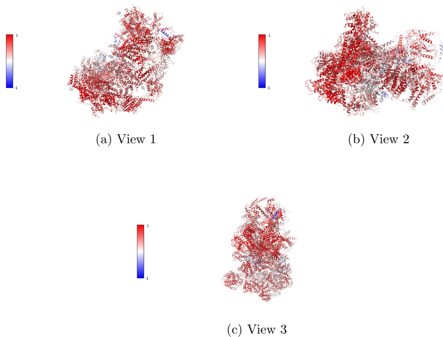
Figure 19: Atomic model colored by DAQ Views generated by ChimeraX at the following X, Y, Z angles: View 1 (0, -90, -90), View 2 (-90, 0, -90), View 3 (0, 0, 0).
