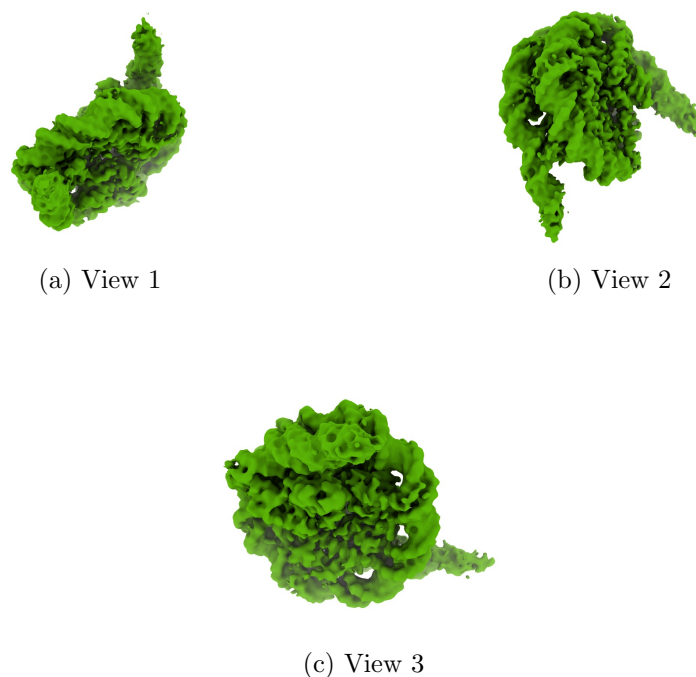
Figure 4: Isosurface at threshold=0.012400. Views generated by ChimeraX at a the following X, Y, Z angles: View 1 (0, -90, -90), View 2 (-90, 0, -90), View 3 (0, 0, 0).
