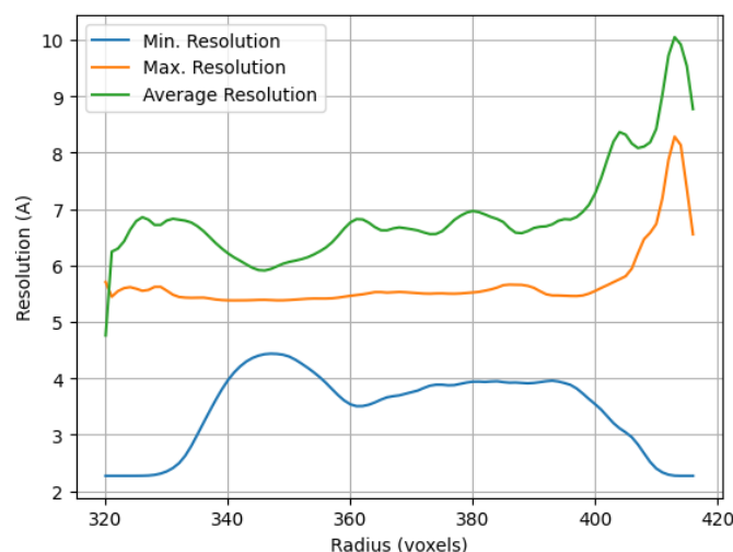
Figure 26: Radial averages (in space) of the minimum, maximum and average resolution at each voxel.
