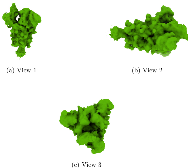
Figure 4: Isosurface at threshold=0.400000. Views generated by ChimeraX at the following X, Y, Z angles: View 1 (0, -90, -90), View 2 (-90, 0, -90), View 3 (0, 0, 0).
