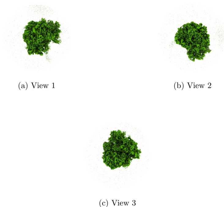
Figure 4: Isosurface at threshold=0.335000. Views generated by ChimeraX at a the following X, Y, Z angles: View 1 (0, -90, -90), View 2 (-90, 0, -90), View 3 (0, 0, 0).
