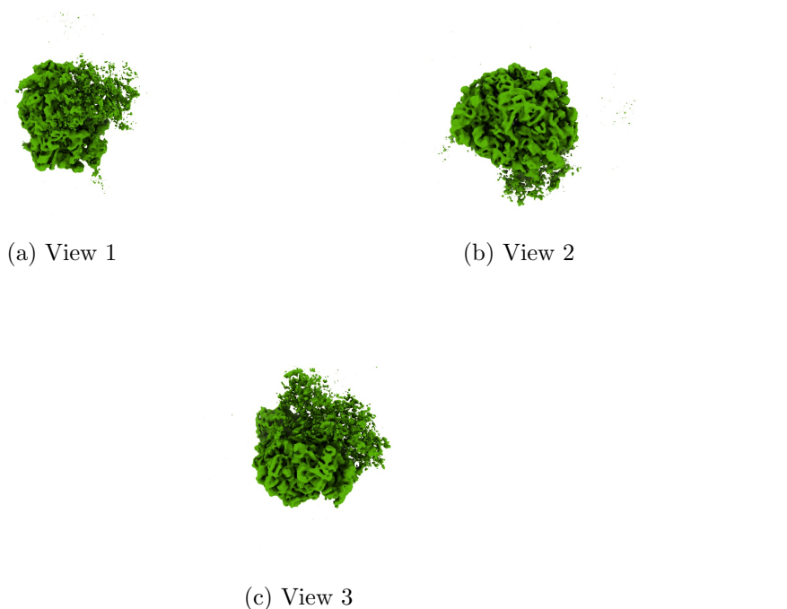
Figure 4: Isosurface at threshold=0.124000. Views generated by ChimeraX at a the following X, Y, Z angles: View 1 (0, -90, -90), View 2 (-90, 0, -90), View 3 (0, 0, 0).
