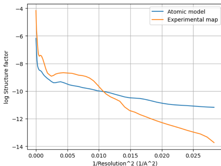
Figure 14: Guinier plot of the atom model and experimental map. The X-axis is the square of the inverse of the resolution in Å.
