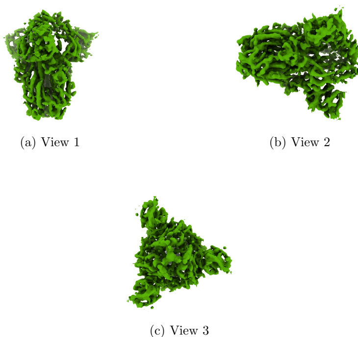
Figure 4: Isosurface at threshold=0.399000. Views generated by ChimeraX at a the following X, Y, Z angles: View 1 (0, -90, -90), View 2 (-90, 0, -90), View 3 (0, 0, 0).
