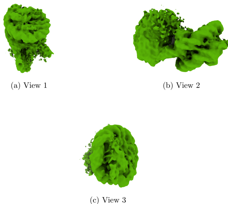
Figure 4: Isosurface at threshold=0.052000. Views generated by ChimeraX at a the following X, Y, Z angles: View 1 (0, -90, -90), View 2 (-90, 0, -90), View 3 (0, 0, 0).
