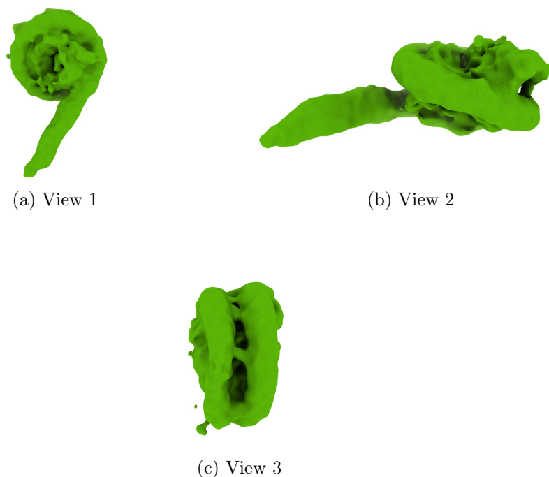
Figure 4: Isosurface at threshold=0.052000. Views generated by ChimeraX at a the following X, Y, Z angles: View 1 (0, -90, -90), View 2 (-90, 0, -90), View 3 (0, 0, 0).
