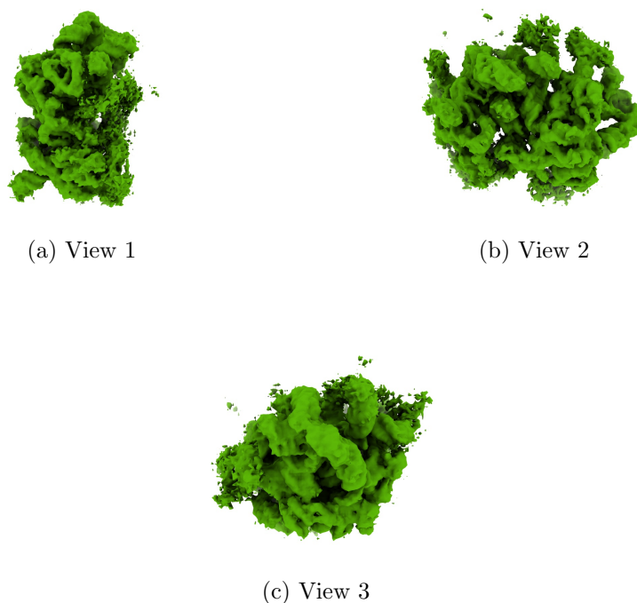
Figure 4: Isosurface at threshold=0.002500. Views generated by ChimeraX at a the following X, Y, Z angles: View 1 (0, -90, -90), View 2 (-90, 0, -90), View 3 (0, 0, 0).
